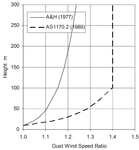
Figure B-2 Differences in elevation adjustment of peak gust speeds.
