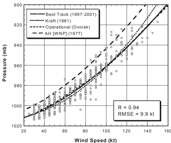
Figure 3.18 Pressure – wind relationships based on best track data in the Atlantic from Brown and Franklin (2002); 1 min winds shown.
