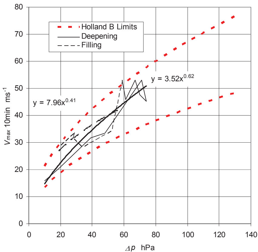
Figure 4.6 Wind-pressure development of Hurricane Michelle , October 2001.
